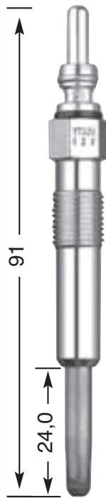
Y-732 U M 10 x 1.0 10 Hex 12 V DP 4
