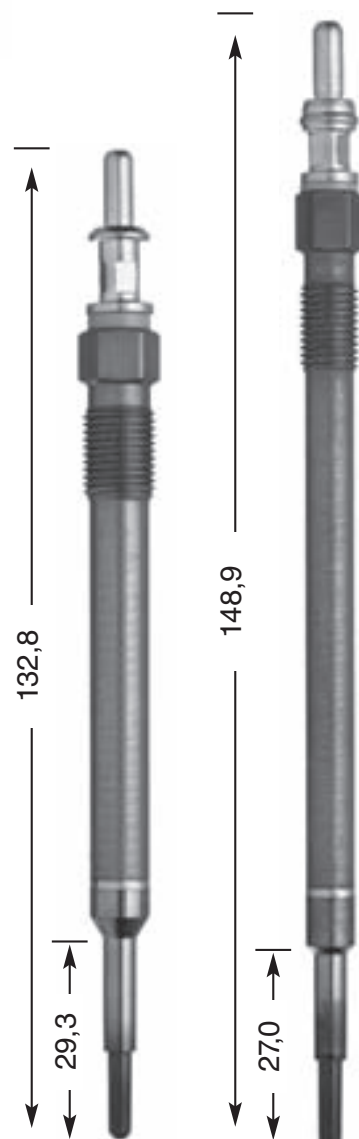
CZ 106 M 10 x 1.0 10 Hex 7 V DP 53
