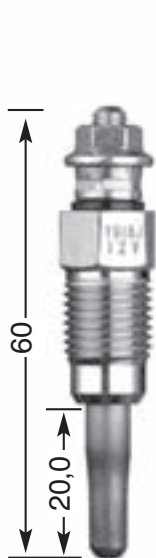
Y-918 J M 12 x 1.25 12 Hex 12 V DP 2
