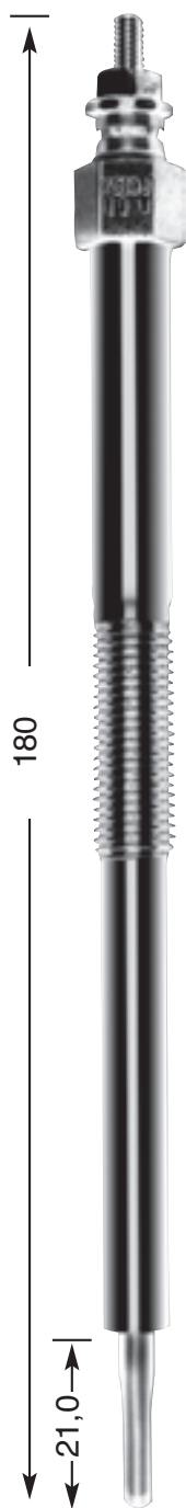
Y-519 J M 12 x 1.0 10 Hex 11 V DP 61
