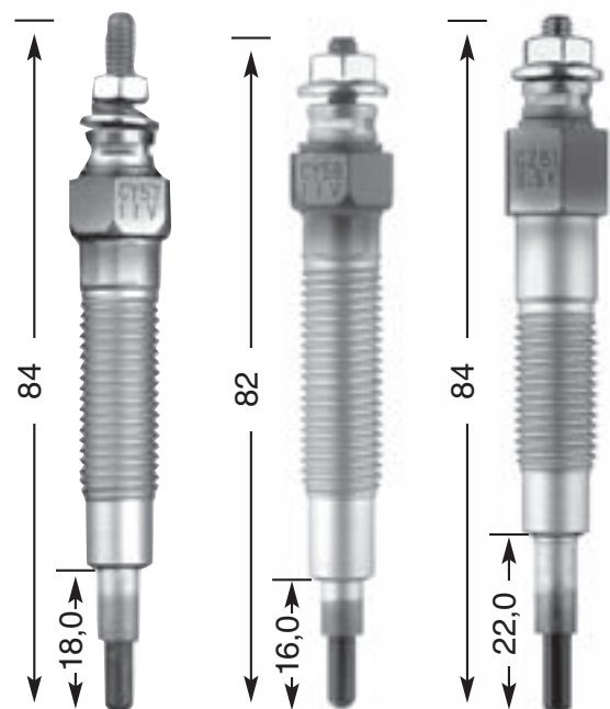
CY 57 M 10 x 1.25 12 Hex 11 V DP 21
