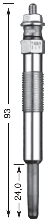
Y-506 R M 10 x 1.0 10 Hex 11 V
