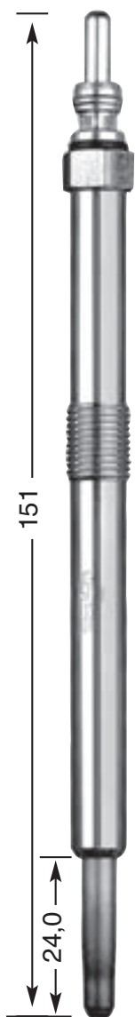
Y-517 J M 10 x 1.0 10 Hex 11 V
