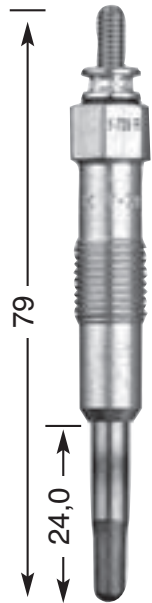
Y-739 R M 10 x 1.0 10 Hex 11 V
