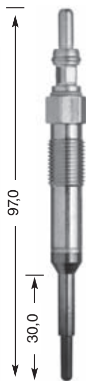
CZ 104 M 10 x 1.0 10 Hex 7 V DP 52
