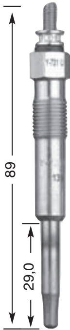
Y-731 U M 10 x 1.0 10 Hex 11 V DP 9
